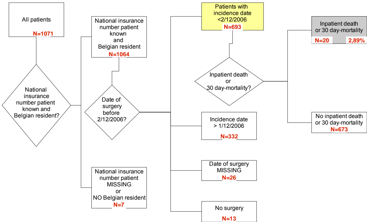
Figure 43. Algorithm for QI 1234 (prospective database).
